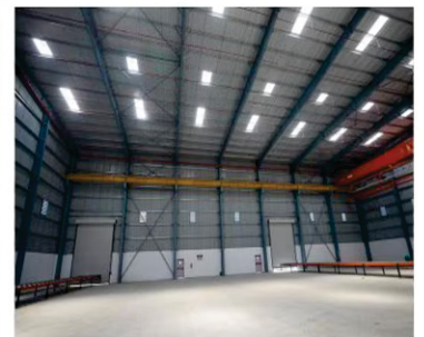
In Side View of PEB Shade
